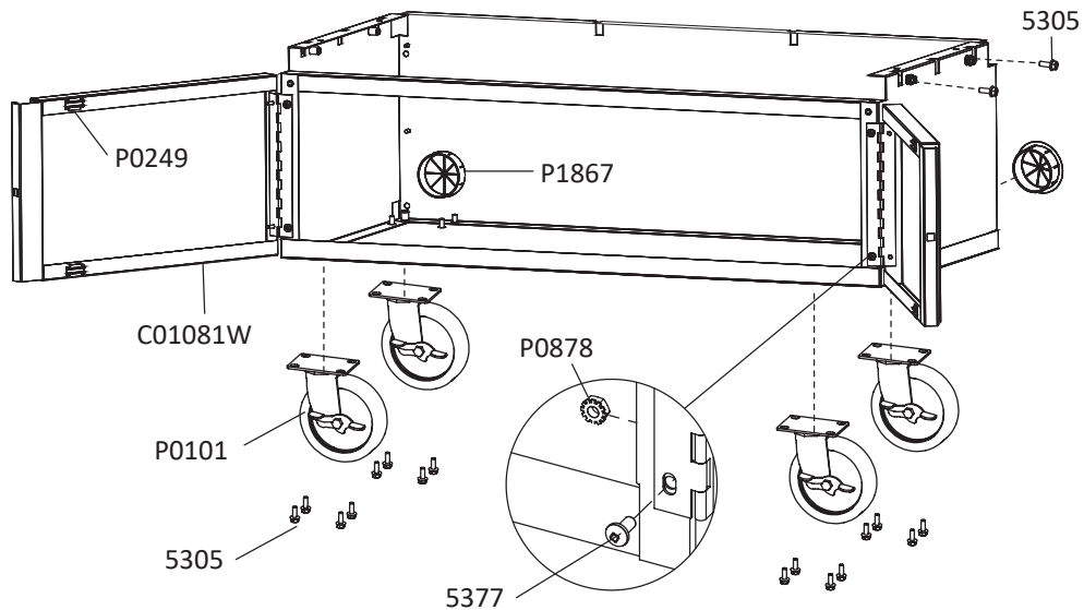
SA0368 Peripheral Cabinet Base
